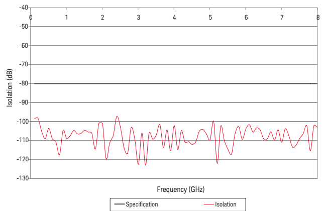
Figure 7. P9402A isolation vs. frequency (typical)
