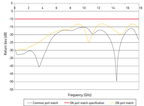
Figure 9. P9402C return loss (ON) vs. frequency (typical)
