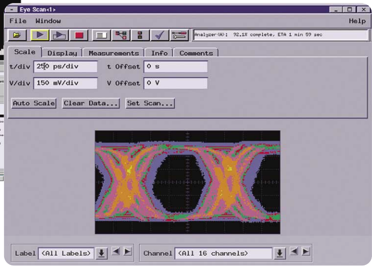
Figure 8. Identify problem signals quickly by using eye scan to make eye diagram measurements on up to hundreds of signals simultaneously.
